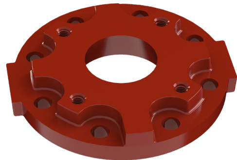
3" ANSI side featuring threaded 3" ANSI pattern and clearance for 5/8" - 11 screw hex heads
